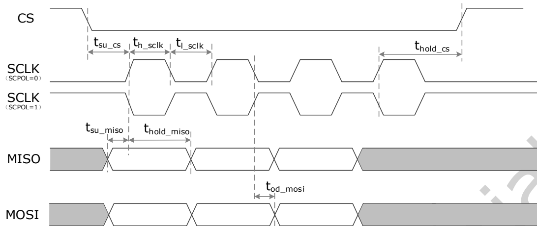
Fig.4-11 SPI interface master mode timing
