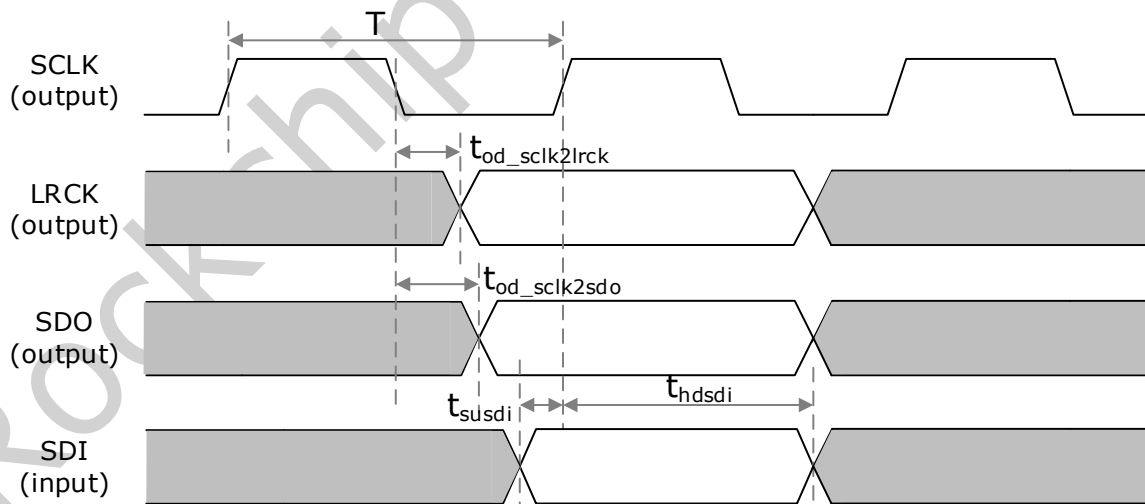
Fig.4-7 SAI interface master mode timing
